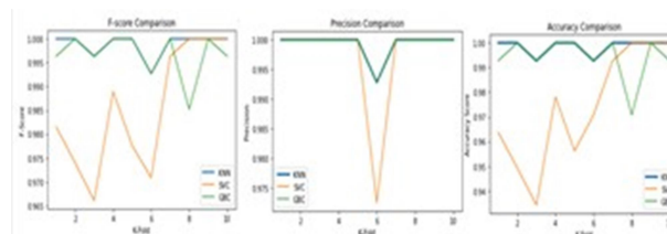
Fig.8 Algorithm Comparison
