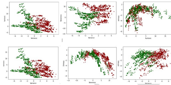
Fig.5 features comparison
