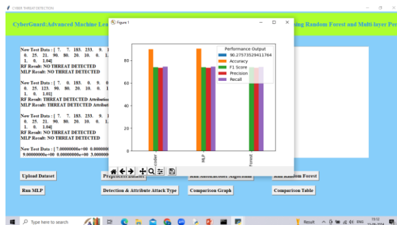
Fig.7.8 Algorithms Graph
