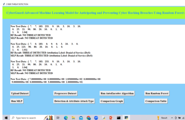
Fig.7.7 Threat Detection
