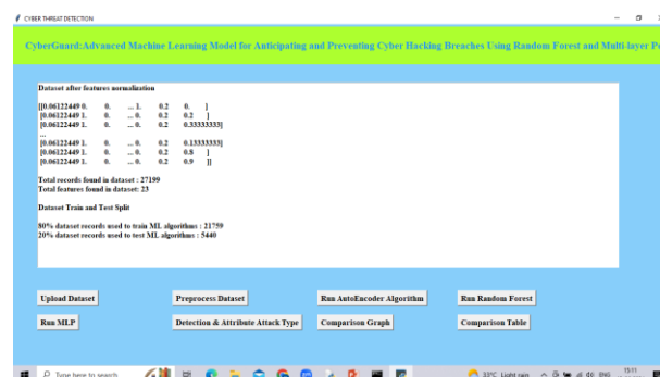
Fig.7.2 Data Preprocessing
