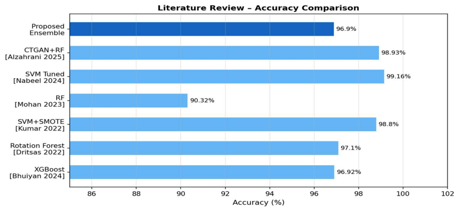
Figure 3: Accuracy Comparison of Related Works vs. Proposed System
