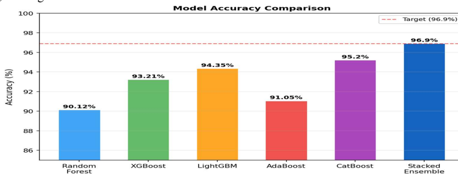
Figure 9: Accuracy Comparison Bar Chart – All Models
