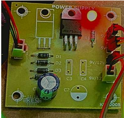
fig 6 Voltage Regulator
