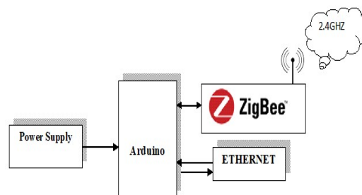
Block Diagram of Monitoring Section
