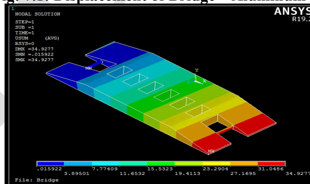
Fig: 7.2: Displacement of Bridge – Duralumin
