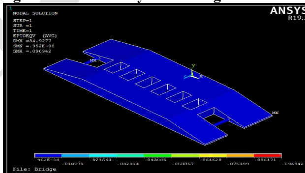
Fig: 7.6: Strain Analysis of Bridge – Duralumin
