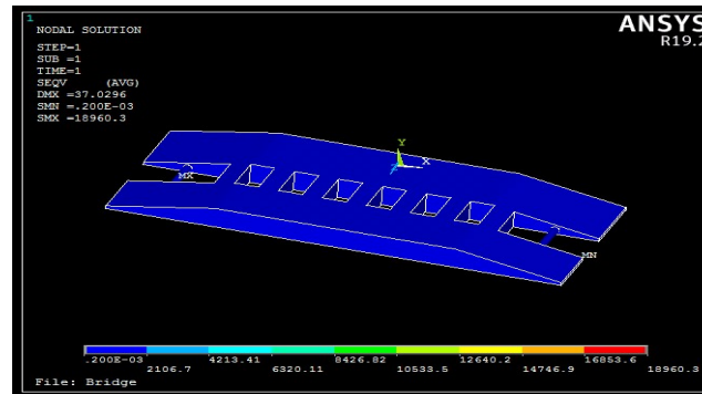
Fig: 7.3: Stress Analysis of Bridge – Aluminum
