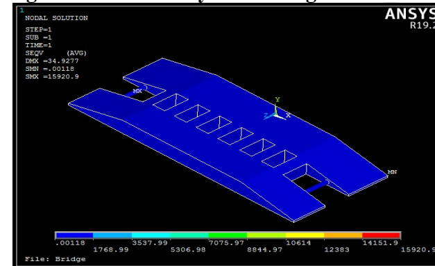
Fig: 7.4: Stress Analysis of Bridge – Duralumin
