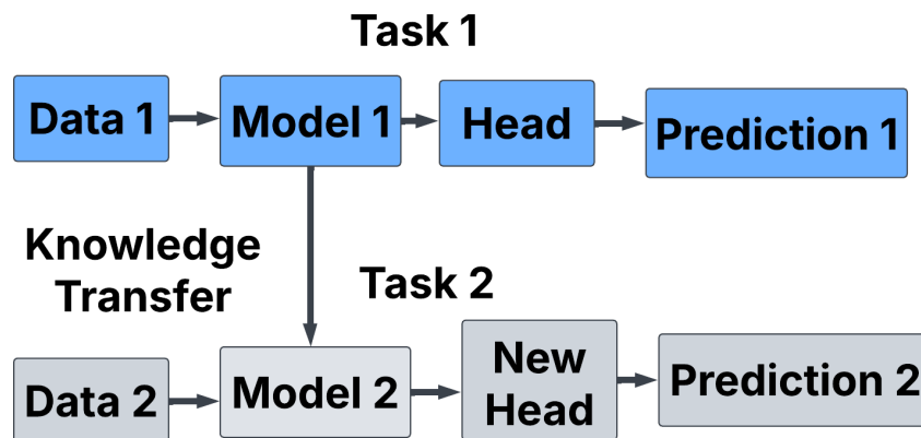
Figure 2. Knowledge Transfer for Multi-Task Learning
