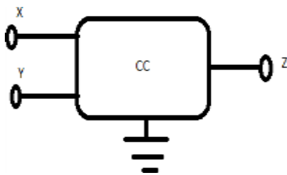
Fig. 2. Block diagram current conveyor
