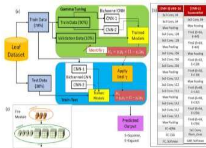
Figure2 workflow bi-channel Convolution Neural Network (a) workflow (b) CNN-1 and CNN-2(c) SqueezeNet's FireModule networks
